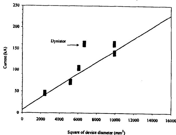
Figure 5. Results of experimental tests on symmetric thyristors with diameters of 50 to 100 mm to determine their failure levels. The dynistor is asymmetric and has a highly interdigitated drive structure and a high current drive.
