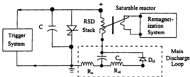
Figure 7. Discharge circuit for evaluation of MPG-2. C_o is 200 \mu F, R_o (load) is 143 m \Omega . The reverse clipper circuit consists of a resistance R_{cl} of 34 m \Omega and a diode D_{cl} .
