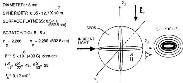
Fig. 3. Characteristics and orientation of LiNbO 3 SEOS. The SEOS orientation was chosen to achieve a low value of V_{\pi}^6 ( \vec{E}_0 = \vec{0} when orienting the sphere). x_3 is the c-axis, and x_2 is an axis normal to the plane containing the c-axis and an axis normal to the c-axis. The LIF is observed by projecting onto a screen.
