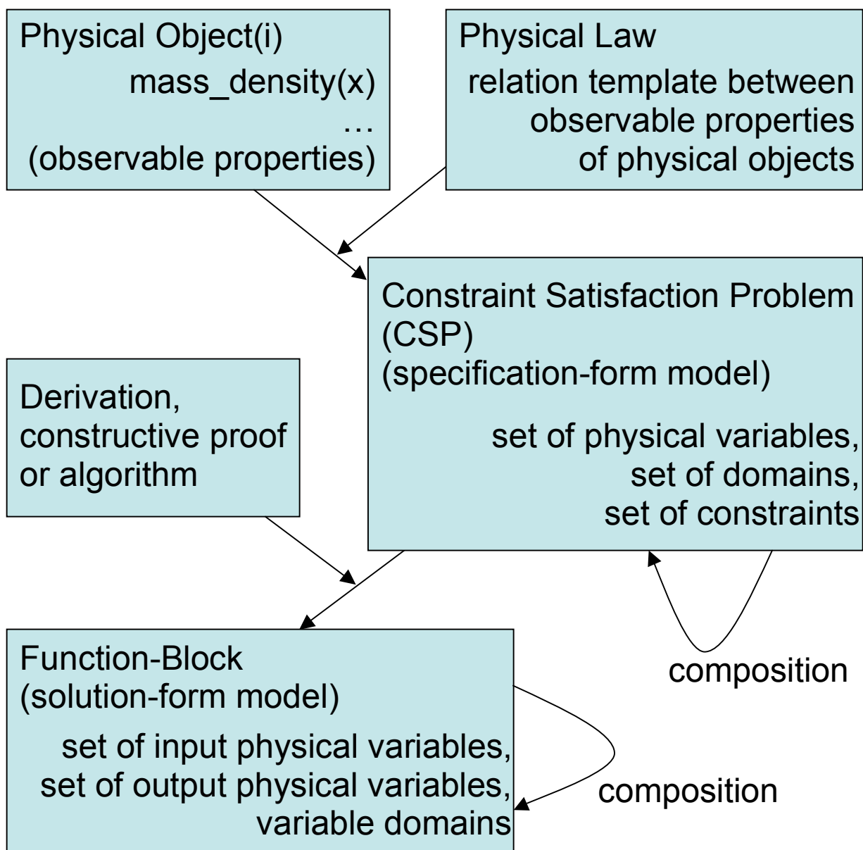
Figure 1. Some semantic concept classes for physics markup
