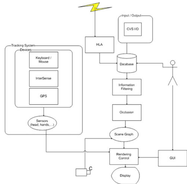
Fig. 6 Software structure of the AR system
