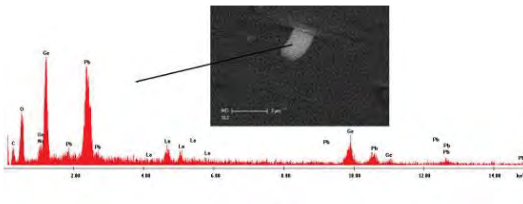
Fig.6. EDX image of KGeF021 (surface scatter).
