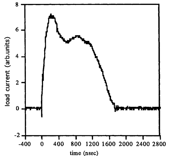
Figure 3. Representative current pulse from test of PFN, indicating \sim 136 nsec risetime and 1.4 \mu\text{sec} FWHM pulsewidth.
