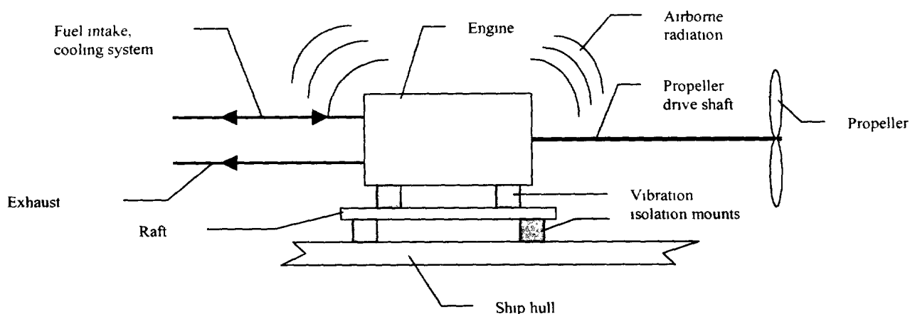
Figure 2.1. Schematics of a Ship Diesel Engine Mounting
