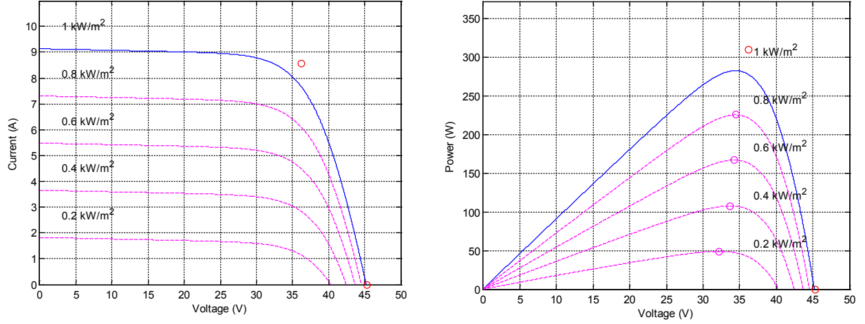
Figure 3.16. Curves for the PV panels used in the model.
