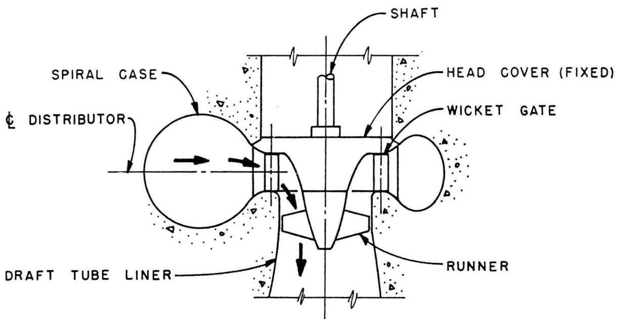
PROPELLER / KAPLAN TURBINE
