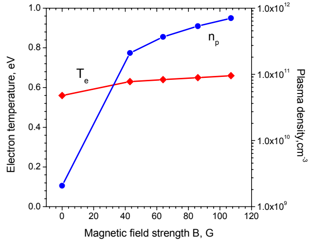
Figure 4. Effect of magnetic field on electron temperature ( T_e ) and plasma density ( n_p ) in Ar plasma. The measurements were performed on axis. Experimental conditions: pressure 50 mTorr, grid voltage 1.3 kV, hollow cathode voltage 360 V.
