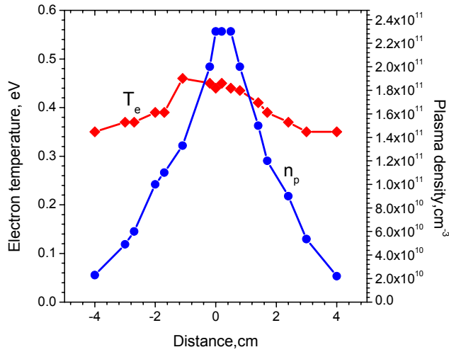
Figure 2. Spatial electron temperature ( T_e ) and plasma density ( n_p ) profiles in argon. Experimental conditions: pressure 20 mTorr, grid voltage 1.3 kV, grid current 19 mA, hollow cathode voltage 360 V, hollow cathode current 35 mA, magnetic field strength 100 G
