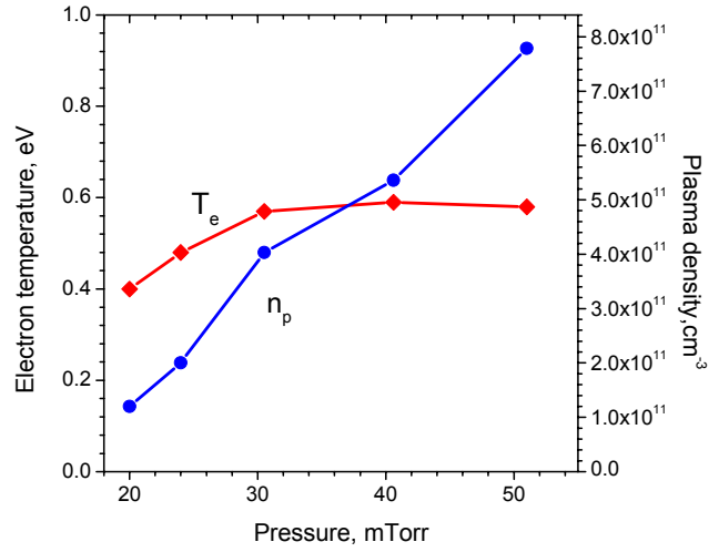
Figure 3. Effect of pressure on electron temperature ( T_e ) and plasma density ( n_p ) in Ar plasma. The measurements were performed on axis. Experimental conditions: grid voltage 1.3 kV, hollow cathode voltage 320 V, magnetic field strength 100 G.
