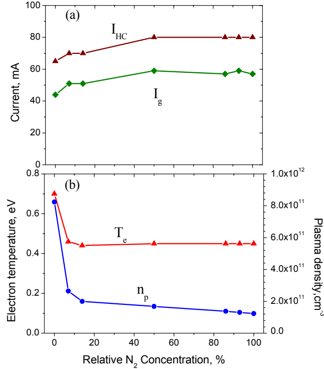
Figure 5. Effect of gas composition on hollow cathode ( I_{HC} ) and grid ( I_g ) currents ( Figure 5a ) and on electron temperature ( T_e ) and plasma density ( n_p ) ( Figure 5b ). The measurements were performed on axis. Experimental conditions: pressure 50 mTorr, grid voltage 1.3 kV, hollow cathode voltage 350 V, magnetic field strength 100 G.
