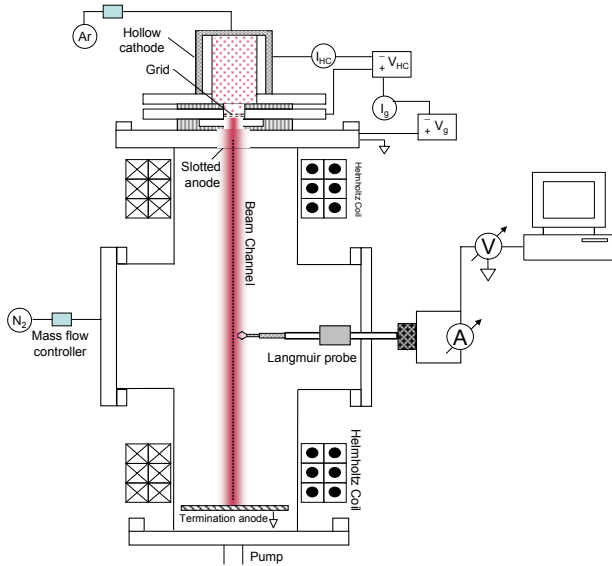
Figure 1. Schematics of the experimental apparatus
