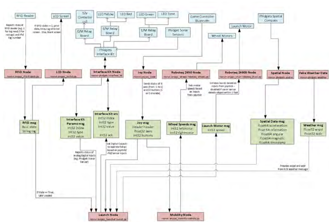
Figure 6.13: ROS communications diagram showing delivered range of functionality for the AMPPS launcher
