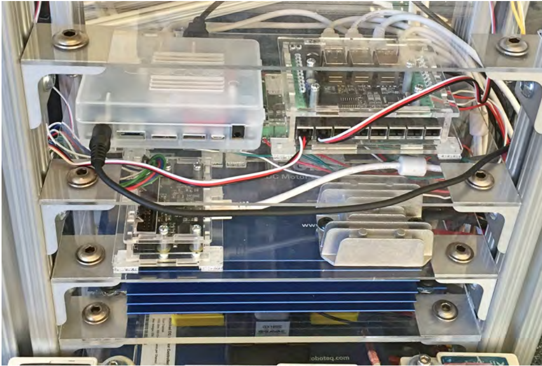
Figure 6.6: AMPPS's embedded ODR0ID XU computer and Phidgets Interface Kit
