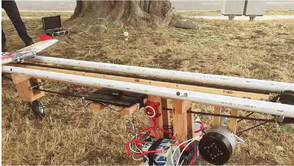
Figure 5.11: Final Chain Launcher system prepared for operational testing
