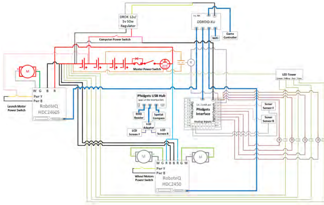
Figure 6.10: Master electrical diagram for the AMPPS
