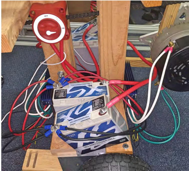
Figure 5.4: Electrical power kill switch for the chain launcher system
