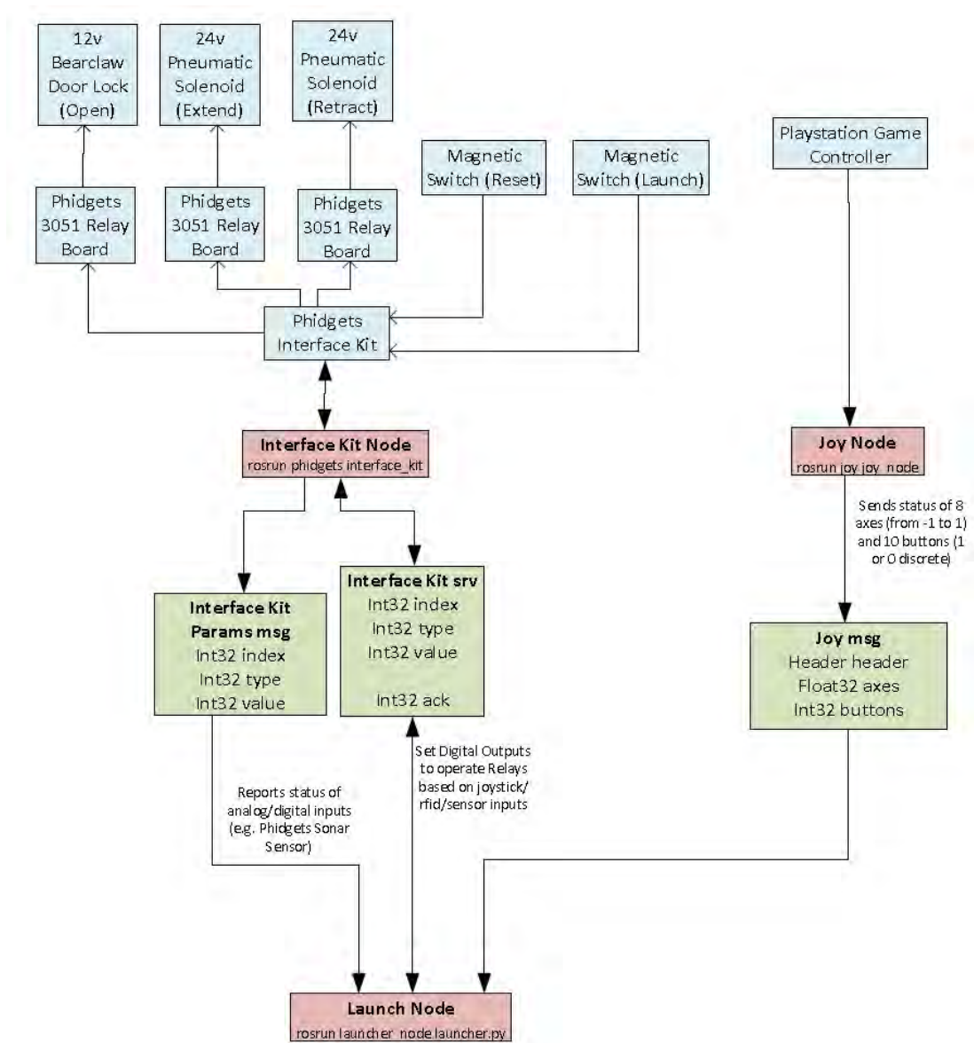
Figure 4.7: ROS communications diagram for the Rapid UAV Launch Engine
