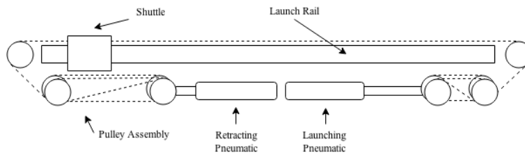
Figure 4.4: Side View of Pneumatic Concept
