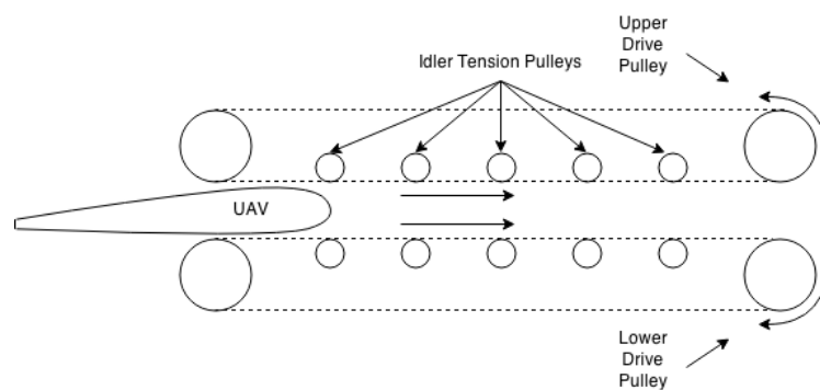
Figure 4.5: Side View of Pitching Machine Concept
