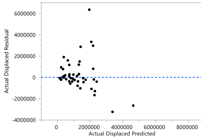
Residual plot for “ Actual Displaced ” Model
