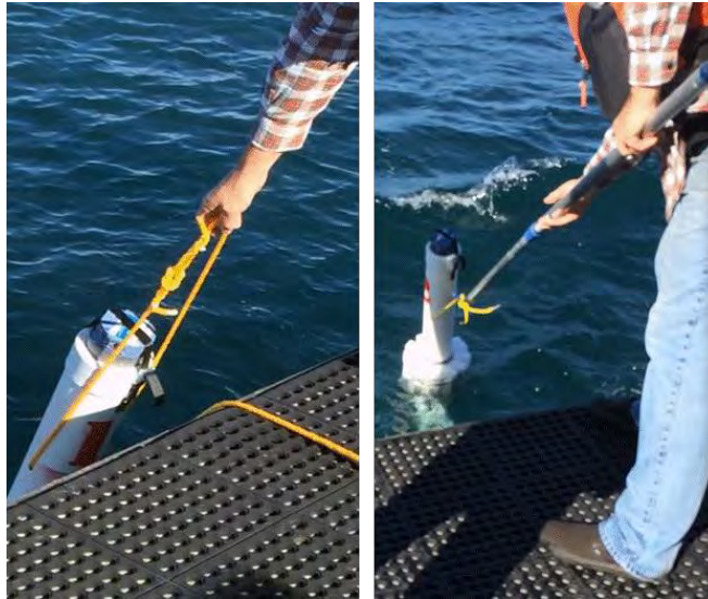
Figure 35. Deployment and Retrieval of a WSB
