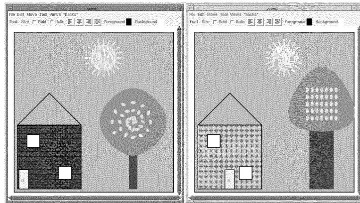
Figure 6.4: Two presentations of the same two-dimensional graphics document, a simple illustration of a house, a tree, and the sun.
