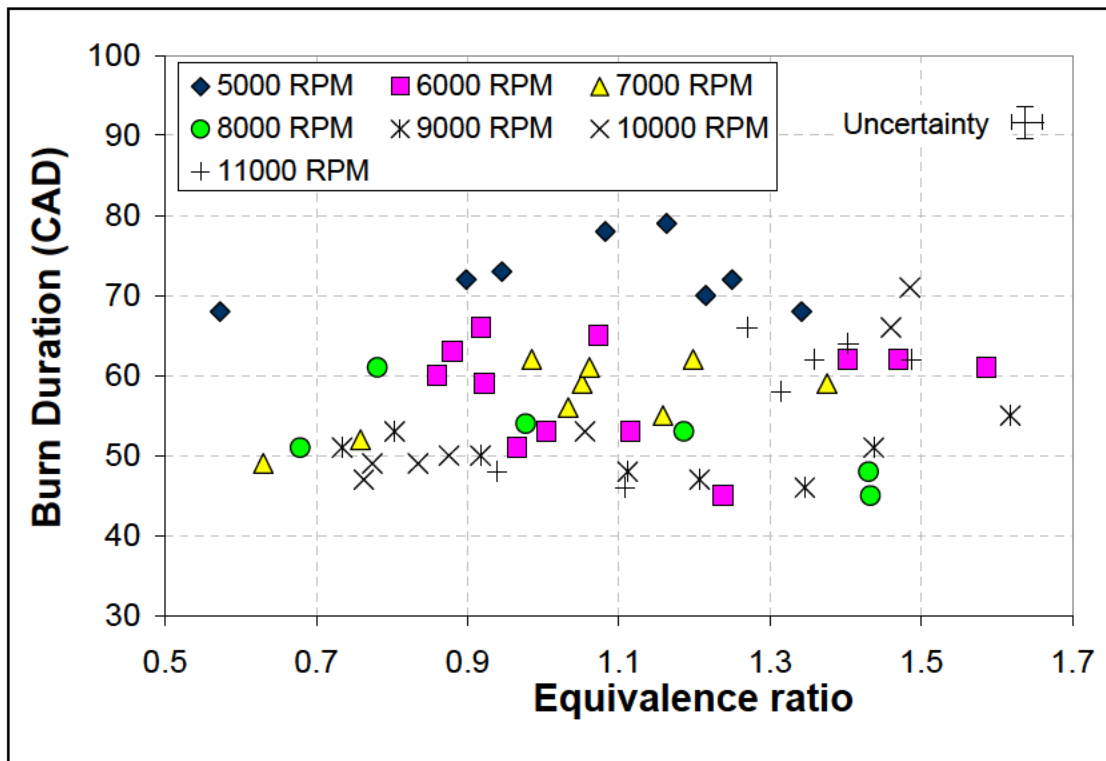
Figure 5–31: Burn duration in crank angle degrees averaged over 50 cycles and plotted as a function of equivalence ratio for the OS 25 FX engine operating at different engine speeds.
