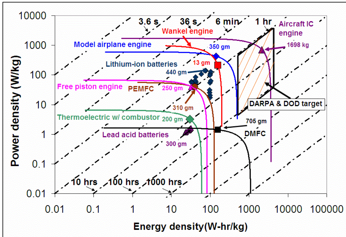
Figure 1–9: Ragone plot of power and energy density with contours of constant endurance comparing different power systems.
