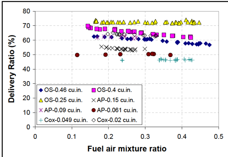
Figure B-2: Delivery ratio at different fuel air mixture ratios and a constant mean piston speed of 4.77 ms -1 for all engines.
