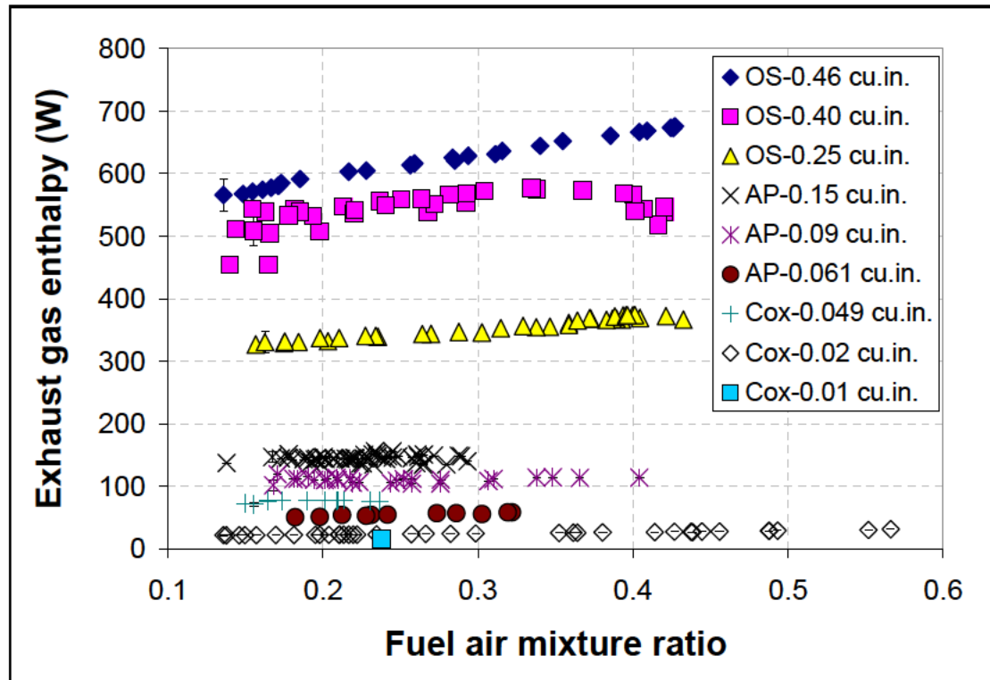
Figure 4–29: Enthalpy released in exhaust for all engines as a function of fuel air mixture ratio at a constant engine speed of 10000 rpm. Error bars are plotted for a single point in each data set and represent average uncertainty for the entire dataset.
