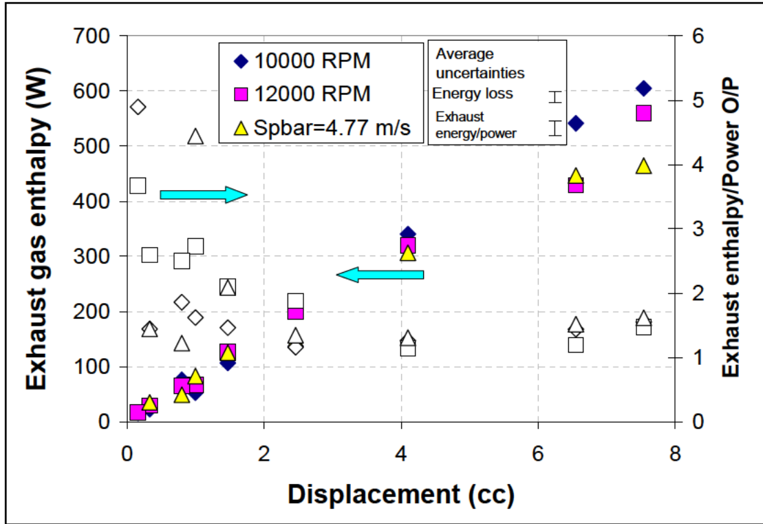
Figure 4–30: Scaling of exhaust enthalpy loss and the ratio of exhaust loss to engine power output as function of engine displacement for two different constant engine speeds of 10000 and 12000 rpm and a constant mean piston speed of 4.77 \text{ ms}^{-1} . All data sets correspond to an equivalence ratio of \sim 1 .
