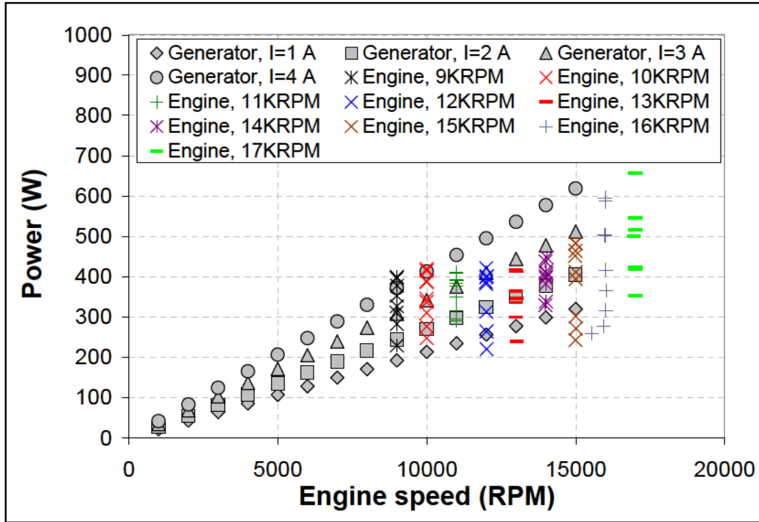
Figure 7–14: Power required by generator to produce different load currents at different operating speeds. Power output from the OS 46 FX engine at different constant engine speeds and fuel–air mixture settings are also presented.
