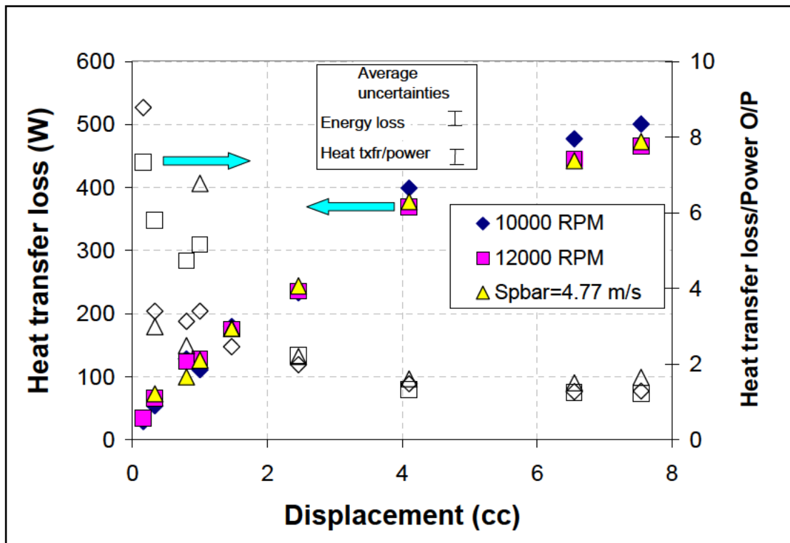
Figure 4–20: Scaling of convective heat transfer losses and ratio of energy loss to engine power output as a function of displacement for two different constant engine speeds of 10000 and 12000
