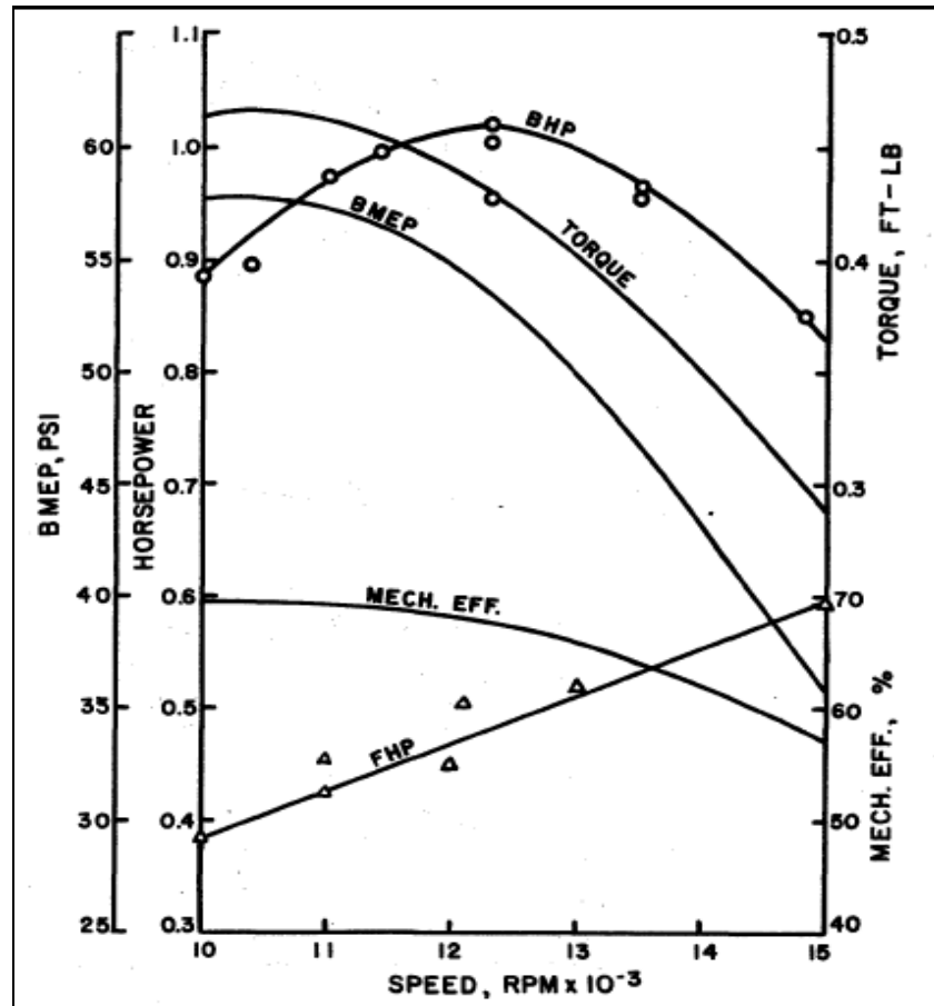
Figure 1-17: Performance data obtained for an engine with displacement 9.95 cc (0.607 cu.in.) with a cylinder head temperature of 477 K (400 °F) and fuel with 67% methanol, 25% oil and 8% nitromethane[70].
