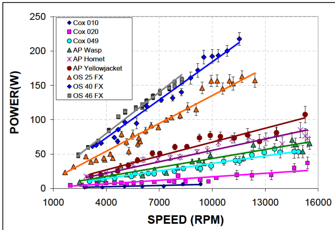
Figure 4-24: Frictional power loss measured from all the engines as a function of engine speed.
