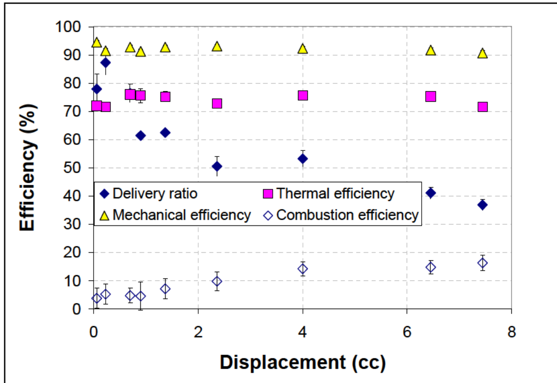
Figure 4–38: Scaling of component efficiencies for all engines as a function of engine displacement at a constant engine speed of 12000 rpm and an equivalence ratio of ~ 1.
