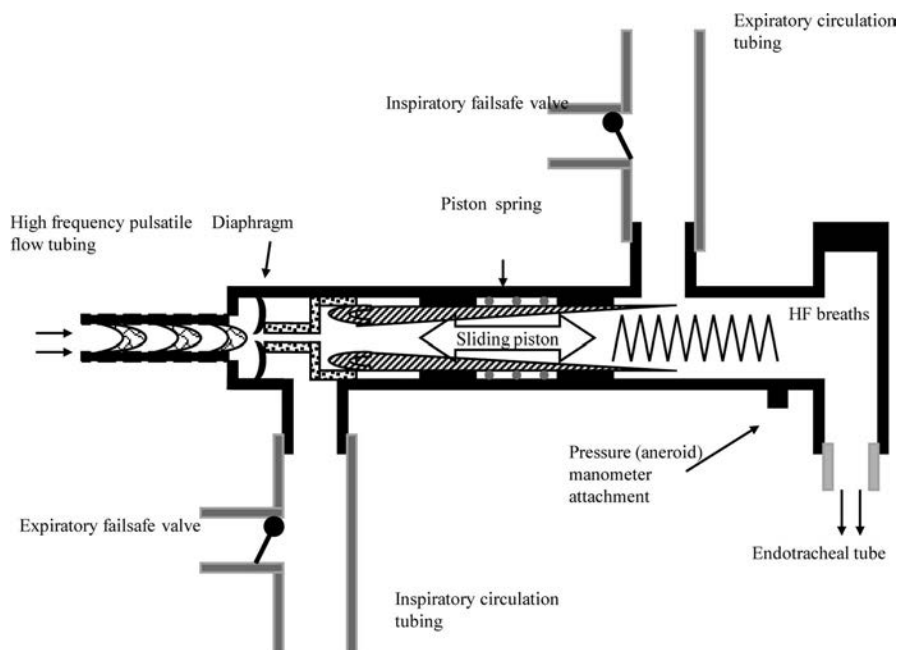
Figure 2. Simplified schematic of the flow amplifier with encased coaxial piston and circulation tubing/fail-safe valve sites. Bidirectional arrow depicts piston motion; HF , high frequency. Reproduced with permission from the American Association of Respiratory Care and Allan and Naworol. 48
