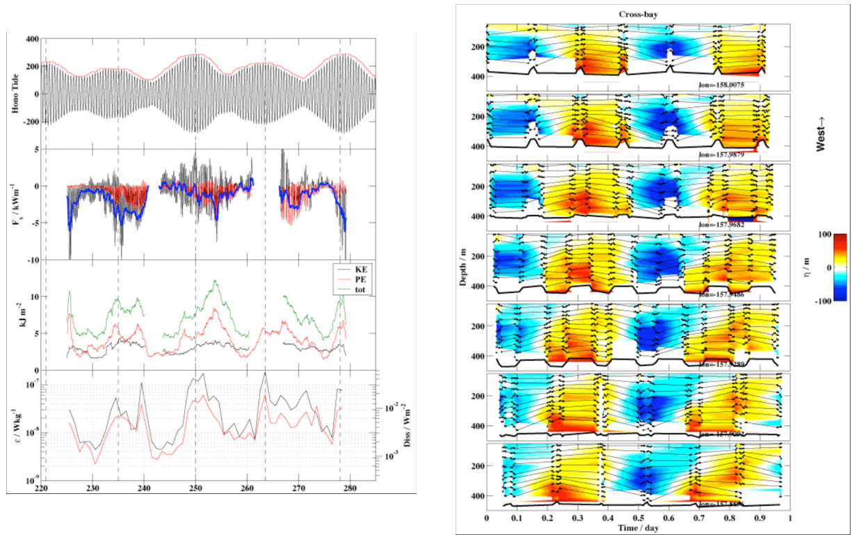
Figure 4 (above left): Time series of depth-average moored quantities. From top: M2 sealevel at Honolulu, eastward energy flux (blue), energy, and dissipation rate from overturns (black). Spring tides are indicated with vertical dotted lines.
