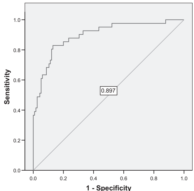
Fig. 3. ROC curve for model derived by logistic regression for prediction of LSIs using ECG-derived variables (SampEn and DFA) and \text{GCS}_{\text{MOTOR}} together. \text{AUC} = 0.897 .
