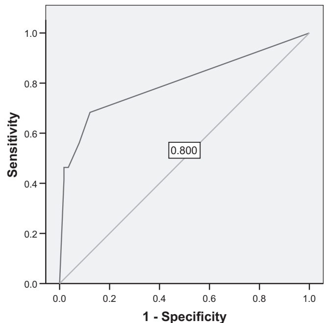
Fig. 2. ROC curve for model derived by logistic regression for prediction of LSIs using the motor component of the Glasgow Coma Scale score ( \text{GCS}_{\text{MOTOR}} ) alone. \text{AUC} = 0.80 .
