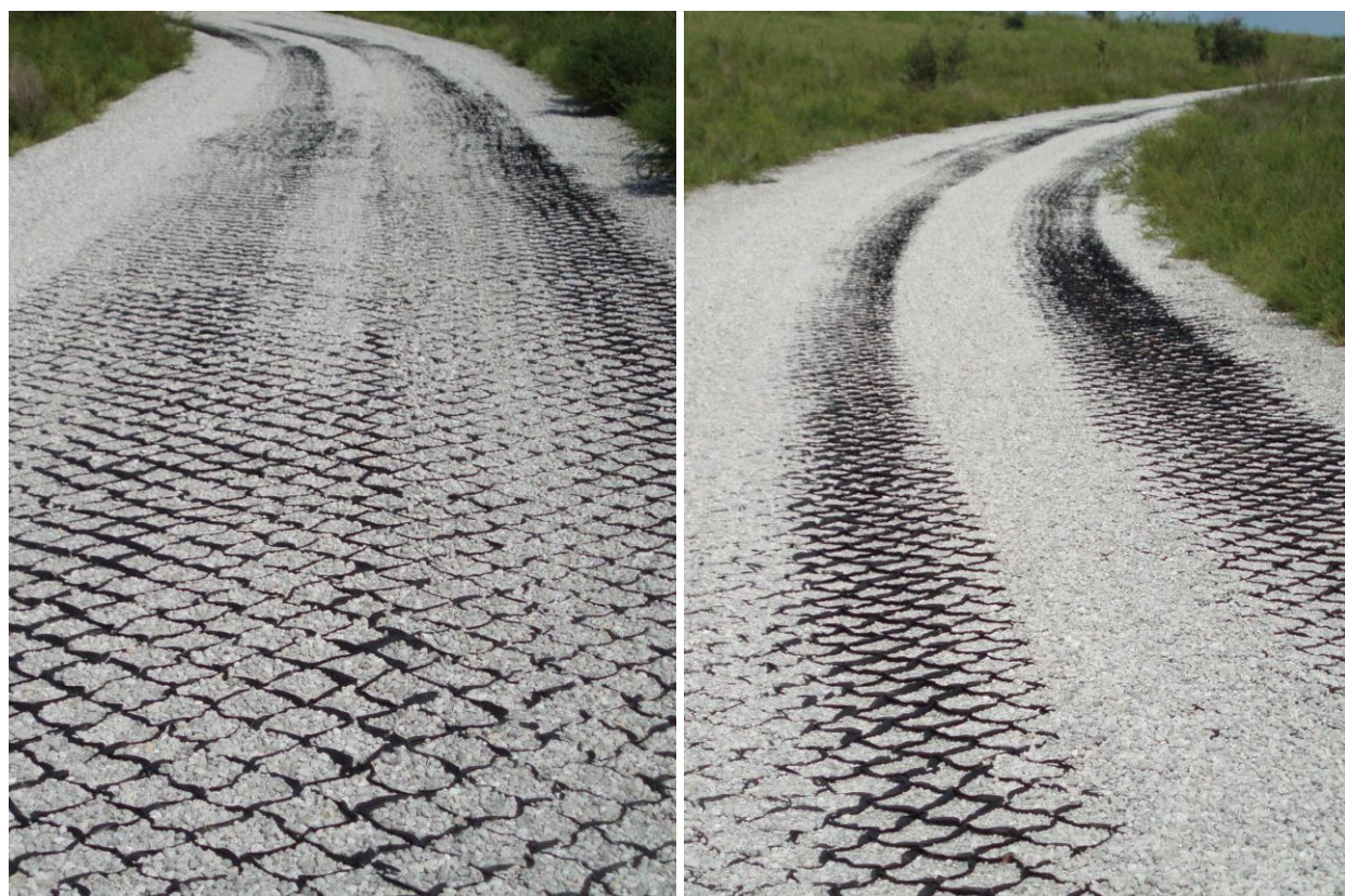
Figure A-10. Crossing Road Approach Damage View Caused by Displacement of Surface Material
