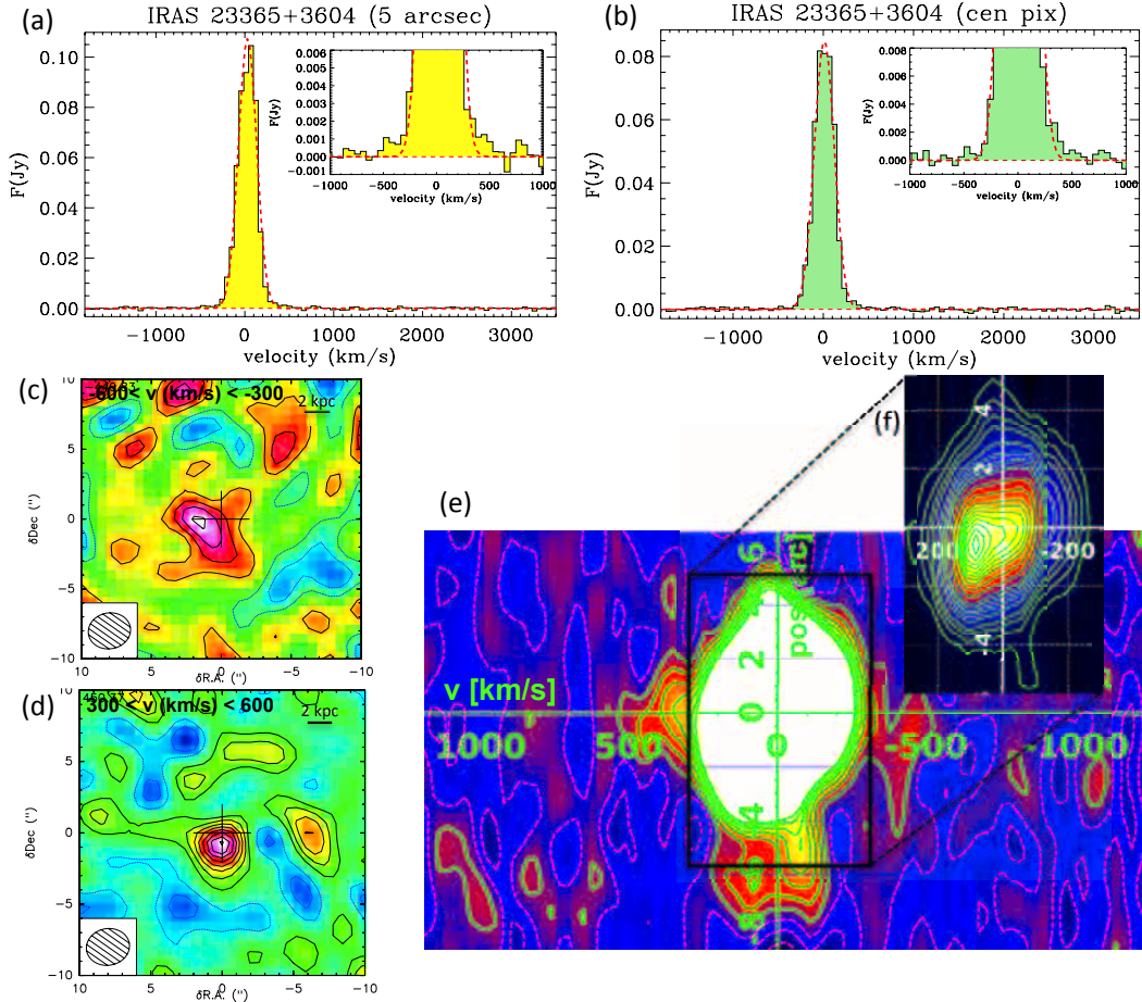
Fig. 3. Continuum-subtracted IRAM-PdBI spectra, maps, and position–velocity diagram of the CO(1–0) emission line of IRAS 23365+3604. Panels a) and b) show the spectra extracted from a circular aperture with a diameter of 5 arcsec and from the central pixel, respectively. For display purposes, the spectra are re-binned in channels of 54 \text{ km s}^{-1} . In both panels the narrow core of the line is fitted with a single Gaussian function (red dashed line). c), d) Cleaned map of the emission integrated in the blue- and red-shifted CO(1–0) wings. Contours correspond to 1\sigma ( 1\sigma rms level of the two maps is 0.2 \text{ mJy beam}^{-1} ). The physical scale at the redshift of the source is 1.232 \text{ kpc arcsec}^{-1} . e) Position–velocity diagram along the major axis of rotation. Inset f) highlights the rotation pattern traced by the narrow component of the CO(1–0) line; this also suggests the presence of a counter-rotating disk visible at large radii (i.e. up to about 8 arcsec from the nucleus, which correspond to \sim 10 \text{ kpc} ). Contours are in steps of 1\sigma (up to 7\sigma ) in panel e) , and 5\sigma in inset f) ; negative contours are in steps of 1\sigma (magenta dashed lines). Each pixel corresponds to 0.6 \text{ arcsec} \times 54 \text{ km s}^{-1} in diagram e) , and to 0.3 \text{ arcsec} \times 27 \text{ km s}^{-1} in the inset f) .
