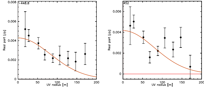
Fig. A.3. Real part of visibilities as a function of the uv distance for the blue (left) and red (right) CO(1–0) wings of IRAS F10565+2448, binned in baseline steps of 20 m. The red curve is the best fit with a circular Gaussian model. The uv tables of the two CO(1–0) wings have been re-centred to their emission centroid positions (obtained from their maps shown in Fig. 2) prior to plotting the uv visibilities in order to correctly estimate their size.
