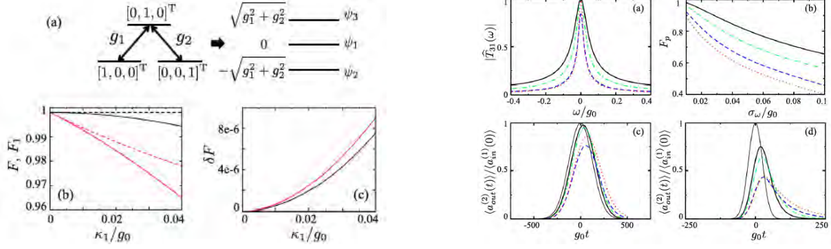
Fig. 3 Left: mechanical dark mode \psi_1 and transfer fidelity for selected Gaussian states. Right: transmission matrix element for traveling photons from the input port of one cavity to the output port of the other.
