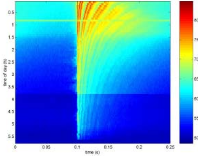
Fig. 4: Measured channel impulse response during the 6-hour drift.
