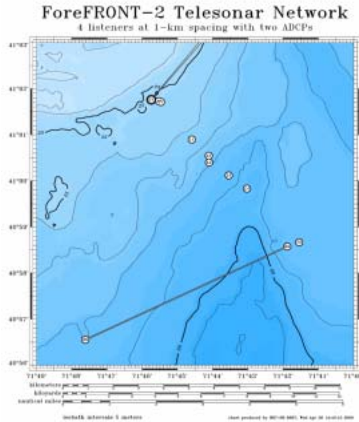
Fig. 3: Bathymetry and drift track during SignalEx-B.
