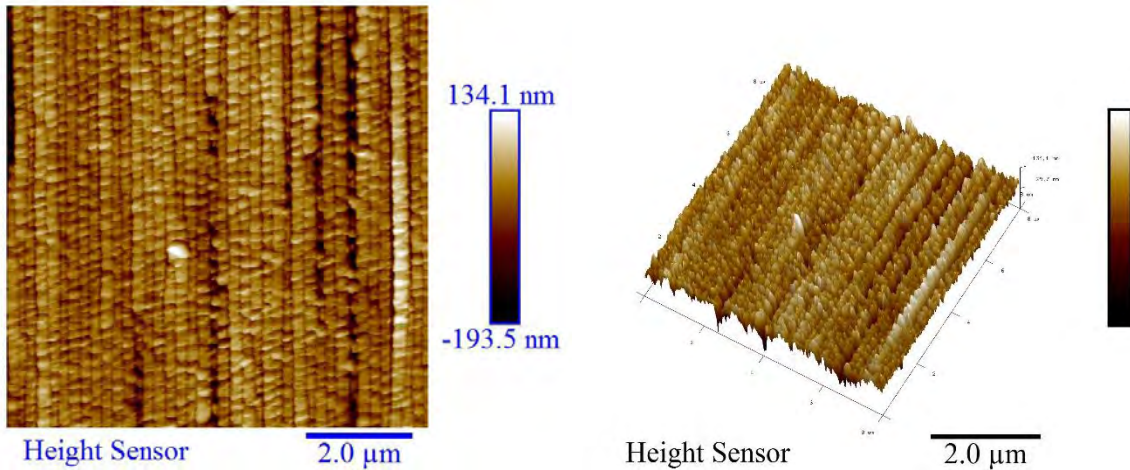
Figure 6. Profile of the nano grating electrode on PMN-PT single crystal.
