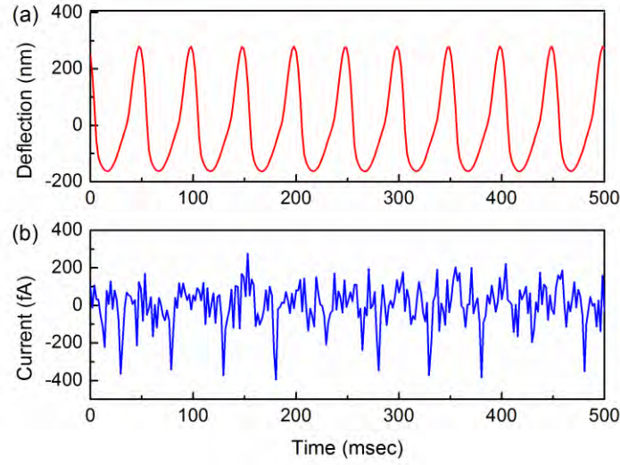
Figure 5. (a) Real time deflection of the PFM probe. (b) Current reading from the pyramid area under 760 nN loading.
