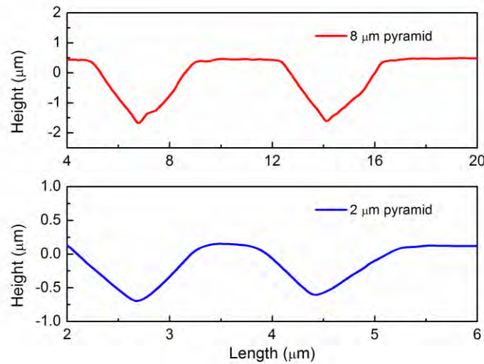
Figure 4. The one dimensional AFM profiles of two nano pyramids with different sizes.
