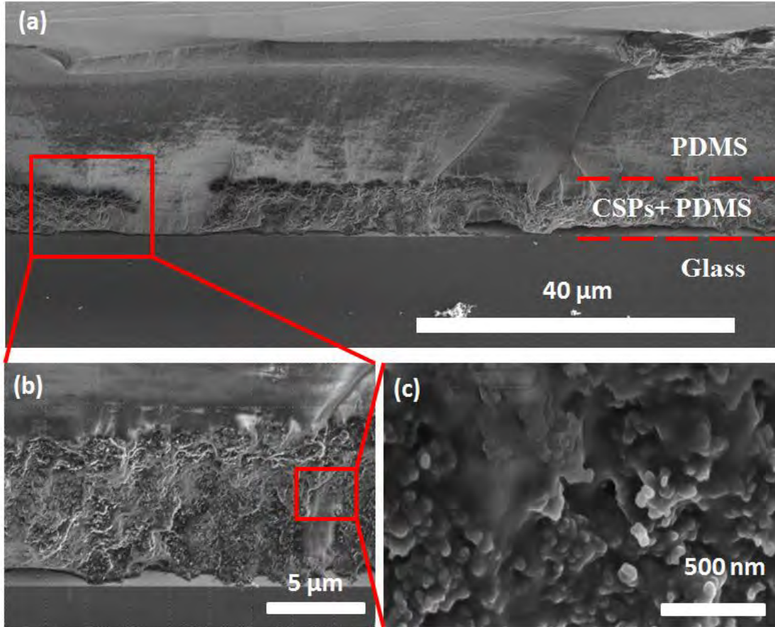
Figure 4. (a) Cross section of CSPs-PDMS composite, and the thickness of PDMS is 18.44 \pm 1.3 \mu\text{m} . (b) The thickness of CSPs-PDMS is 5.99 \pm 0.5 \mu\text{m} , (c) CNPs are well imbedded in PDMS.
