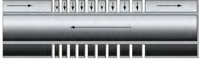
Fig. 2 The helical section replaced by discrete rings of current
