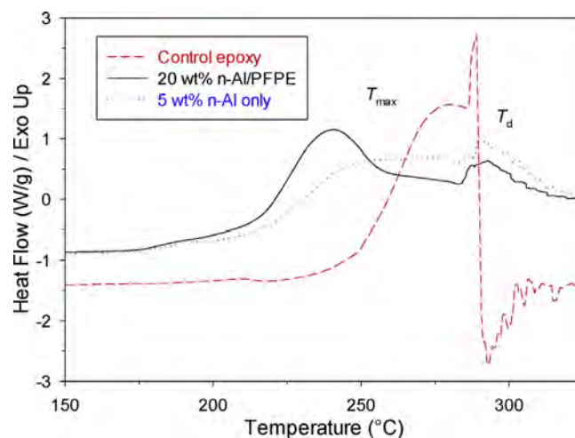
Fig. 3. DSC of the control epoxy without any dopants (red dashes), the epoxide composite loaded with 20 wt% n-Al/PFPE (black solid line), and the epoxide resin loaded with 5 wt% n-Al only, no PFPE (blue dots). (For interpretation of the references to color in this figure legend, the reader is referred to the web version of this article.)
