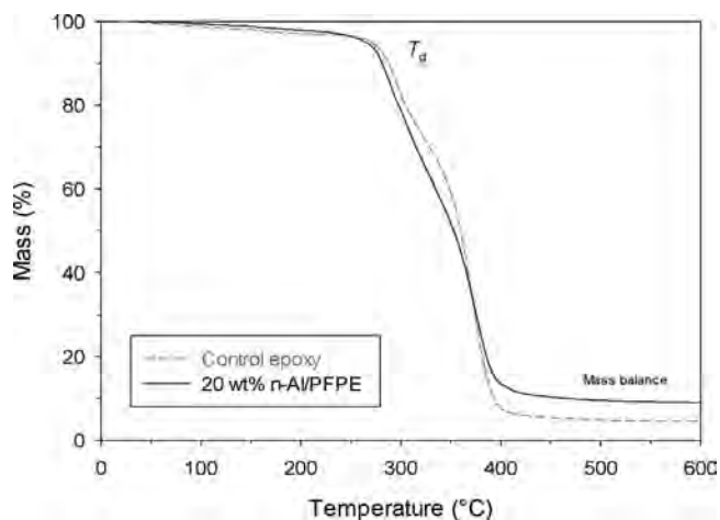
Fig. 5. TGA of the control epoxide without any dopants (red dashes) and the epoxide resin loaded with 20 wt% n-Al/PFPE (black solid line). (For interpretation of the references to color in this figure legend, the reader is referred to the web version of this article.)
