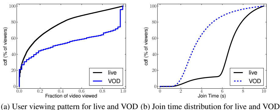
(a) User viewing pattern for live and VOD (b) Join time distribution for live and VOD
