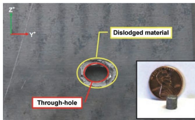
AHEAD sub-projectile and its damage
