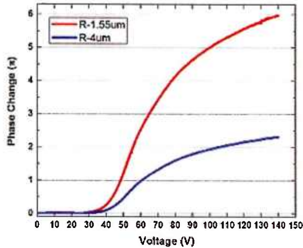
Fig. 18. Voltage-dependent phase change curves in a reflective mode at \lambda=1.5\mu\text{m} and \lambda=4\mu\text{m} .
