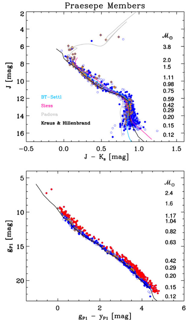
Figure 5. Member candidates in Praesepe selected on the basis of position, proper motion, and magnitude/color. Top: the J vs. J - K_s CMD, together with the stellar models of BT-Settl (Allard et al. 2013; Allard 2014), Siess, Padova, and Kraus & Hillenbrand (2007). Selected stellar mass values are labeled. Symbols are the same as in Figure 4. Bottom: the g_{P1} vs. g_{P1} - y_{P1} CMD for candidates. The solid curve is the main sequence from Kraus & Hillenbrand (2007) transformed to the PS1 system. Red symbols mark possible binaries.
