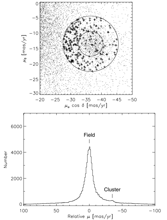
Figure 2. 2MASS/PPMXL stars toward Praesepe. Top: the proper motion distribution. The two circles illustrate the proper motion ranges of \Delta\mu = 4 mas yr ^{-1} and of \Delta\mu = 9 mas yr ^{-1} , respectively. Stars within \Delta\mu = 9 mas yr ^{-1} , but otherwise outside the cluster region (beyond 3^\circ ), and photometrically not following the cluster isochrone, i.e., field stars, are marked with crosses. Bottom: the projected PM distribution along the line connecting the field centroid and the cluster centroid. The bump near -35 mas yr ^{-1} is due to the cluster, which has a standard deviation of 9 mas yr ^{-1} when fitted with a Gaussian function.
