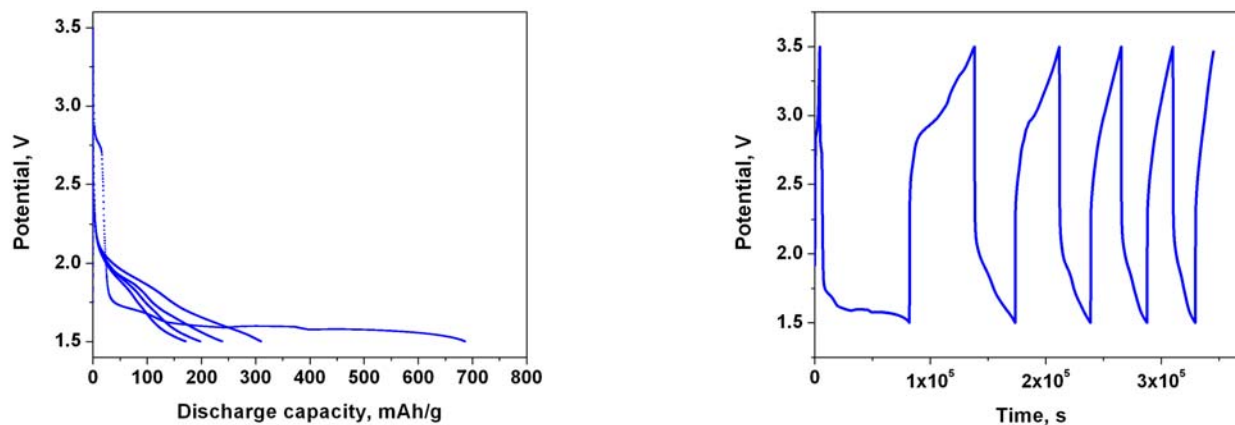
Figure 13: Discharge profiles and capacities of LiPC composites between 3.5 and 1.5 V Li/Li + .
