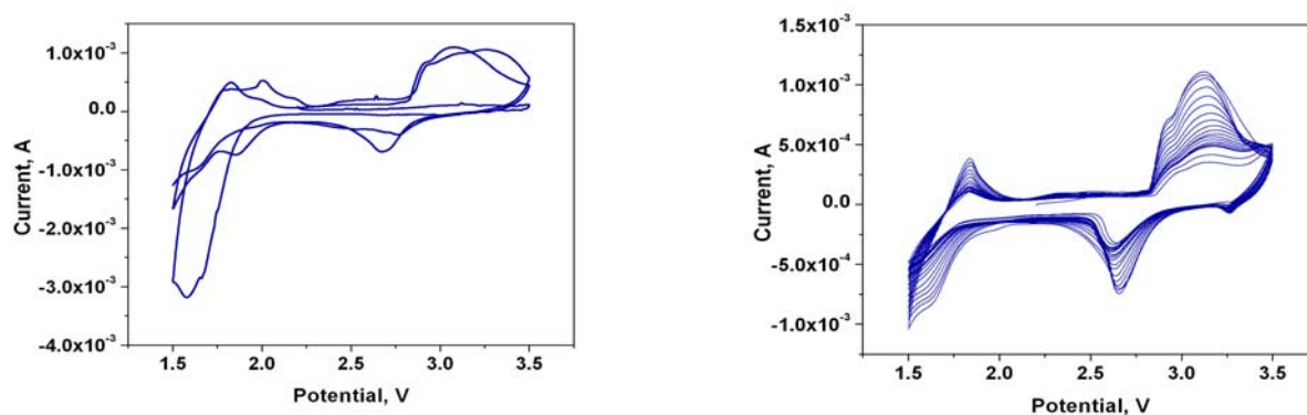
Figure 12: Cyclic voltammograms of LiPC composites in the potential range of 3.5 to 1.5V vs Li/Li + ) at scan rate 2 mV/ sec. The active mass is 3 mg.
