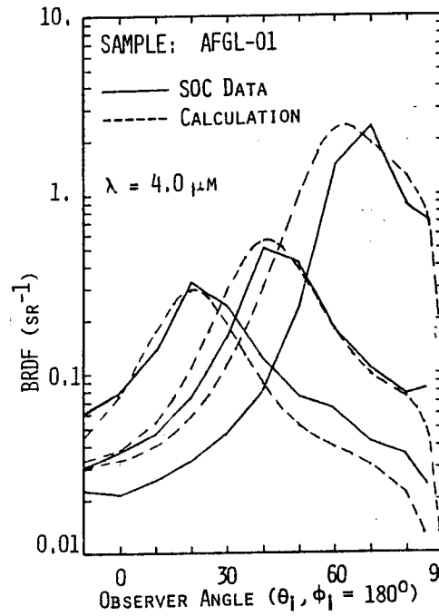
Figure 11. Comparison of Model Calculations (- - -) and SOC Data (—) at 4 \mu\text{m} for sample AFGL-01 for Three BRDF ( \theta_i = 20, 40, 60^\circ ).
