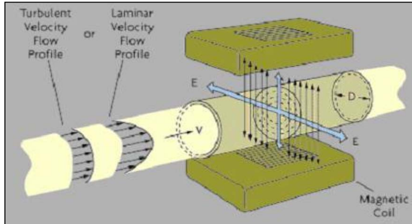
Figure 5-3. Faraday's Law
