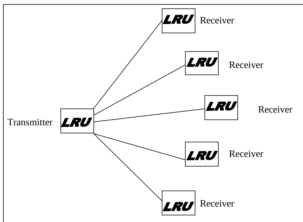
Figure 3-62. Star Topology
