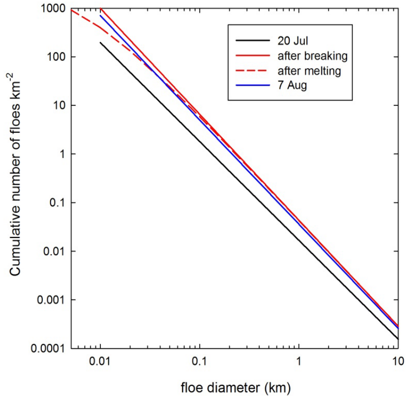
Figure 2. SHEBA major breaking event beginning 20 July (black), analyzed as breaking (solid red) followed by melting (dashed red). The smallest floes post-melting on 7 August have diameters slightly less than 5 m. The power law fit on 7 August (blue) is also shown.
