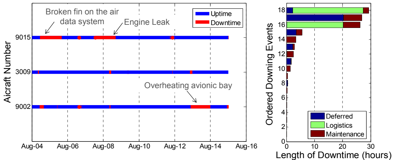
Figure 4-4. AH-64E Downtime during FOT&E I
