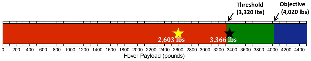
Figure 3-19. AH-64E Lot 4 Hover Payload Performance
