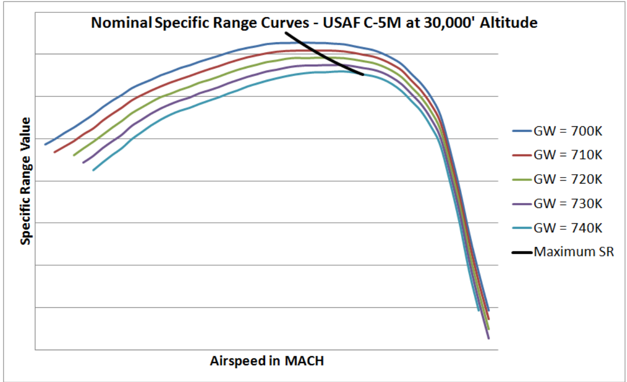
Figure 3 - Nominal Specific Range Curves
