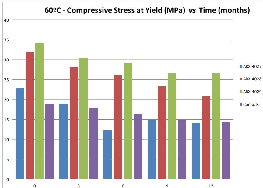
Figure 6: 60 °C ageing profile for compressive stress (MPa)
