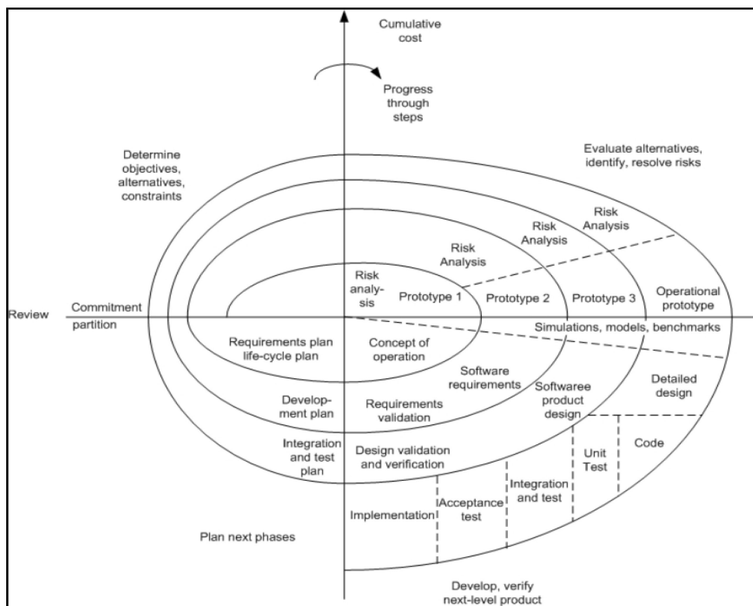
Figure 3-6: The Spiral Model.
