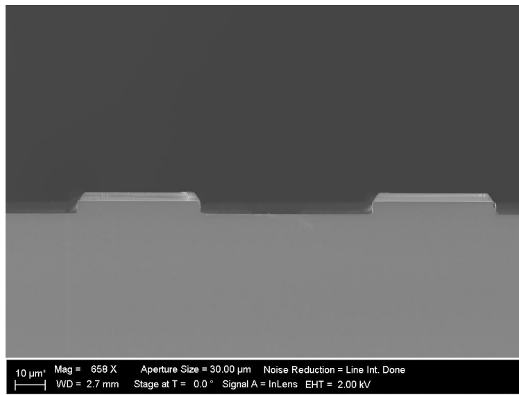
Fig. 3.5 Scanning electron microscope (SEM) image of wafer surface after the top-oxide etch. Dry-etching was used and some etching of the silicon occurred to ensure complete removal of the silicon dioxide. The photoresist mask was removed for the SEM image.
