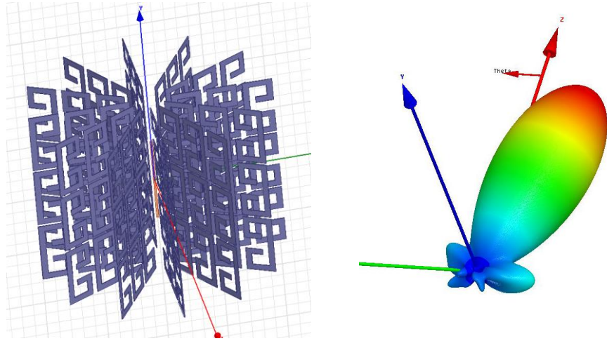
Fig. 5.20 Metamaterial-enhanced dipole using multiple planes of CLL cells and sharp high-gain beam
