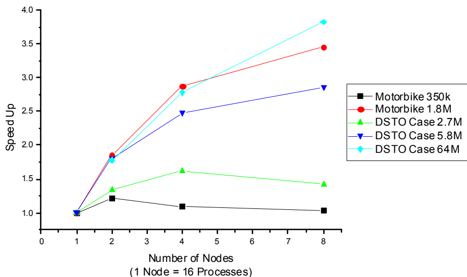
Figure 10 Speedup of each case when run on 1, 2, 4 or 8 nodes of the HPC cluster as per Figure 9
