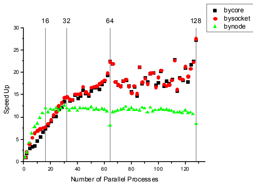
Figure 6 Comparison of process distribution options across a 128 core/8 node cluster
