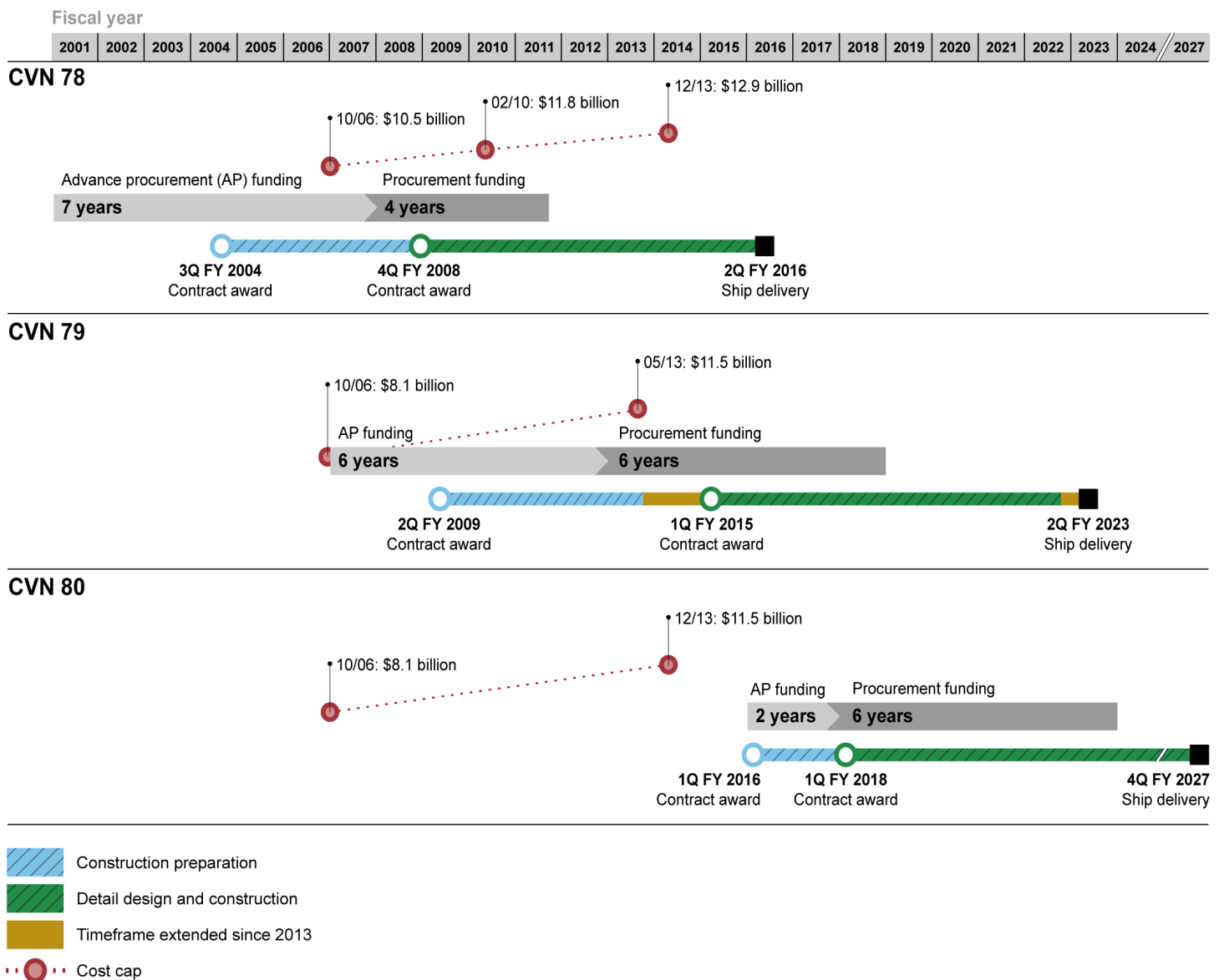
Figure 1: Cost Cap Increases During Acquisition of the Ford Class
