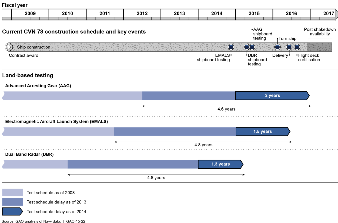
Figure 2: System Developmental Testing Delays
