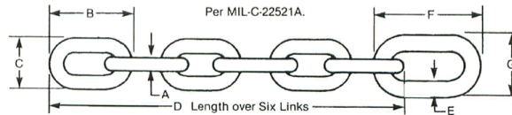
Figure 3: US Coast Guard buoy chain specifications (SST 2012)
