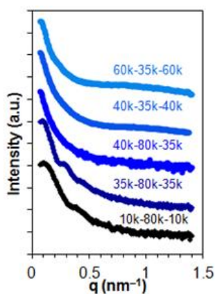
Figure 4. SAXS data at room temperature for PS- b -PVBlm- b -PS triblock copolymers with various molecular weights of the inner PVBlm and outer PS blocks.
