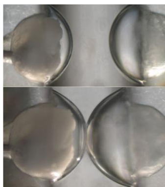
Figure 2: (a) Aqueous droplets before force is applied (b) Aqueous droplets with lipid bilayer formed in between
