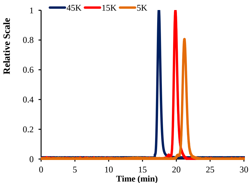
Figure 3. SEC characterization of poly(VBP). 400 MHz, CDCl 3 , 22 °C
