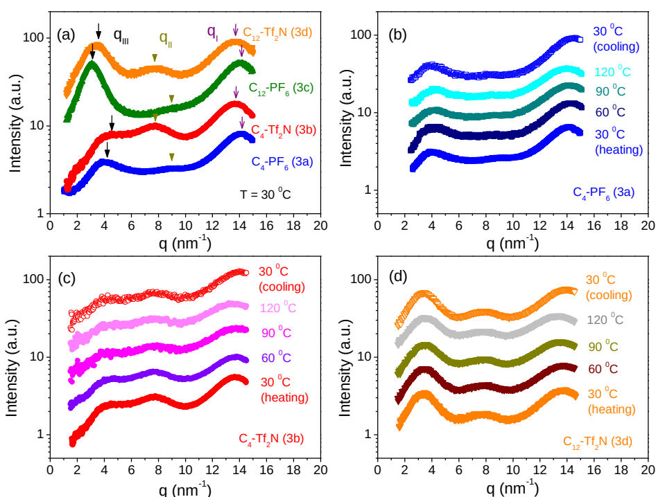
Figure 1 | X-ray scattering intensity as a function of scattering wavevector q for (a) the imidazolium-based ionomers at room temperature and (b) C_4-PF_6 (3a), (c) C_4-Tf_2N (3b) and (d) C_{12}-Tf_2N (3d), each at four temperatures (30, 60, 90 and 120 °C). The arrows indicate peaks that correspond to the amorphous halo ( q_I ), anion-anion correlations ( q_{II} ), and separation between ionic aggregates ( q_{III} ). The intensity of the ionic aggregation spacing peak ( q_{III} ) increases enormously as the tail length increases from n -butyl to n -dodecyl, which we interpret to signify that dodecyl tails favor ion aggregation. The data were shifted on the log intensity scale for clarity.
