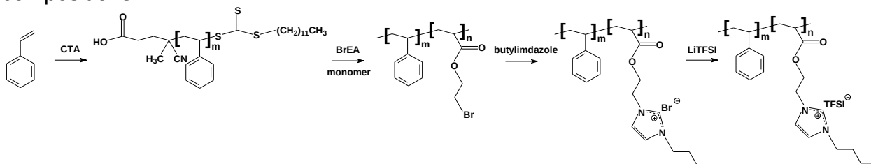
Scheme 1. Synthesis of styrene-containing and acrylate-based PIL block copolymers.
