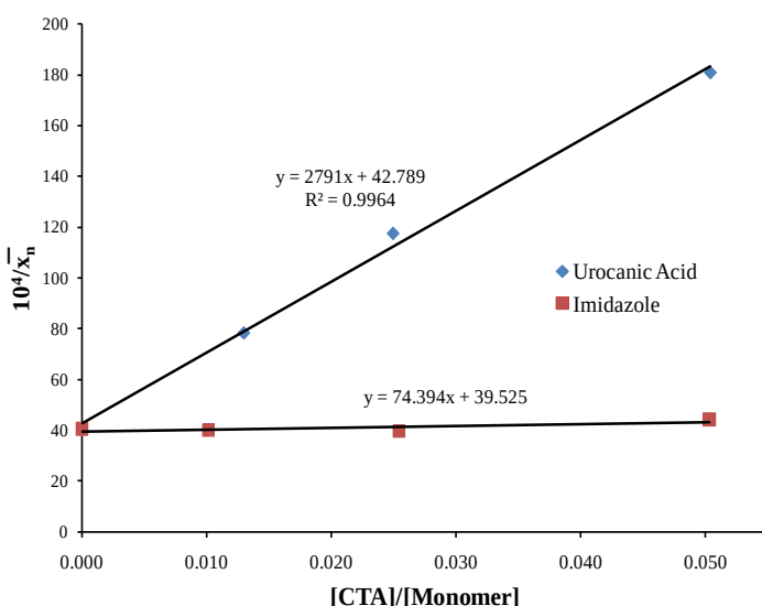
Figure 4. Chain transfer study using urocanic acid and imidazole in a 1-vinylimidazole homopolymerization.
