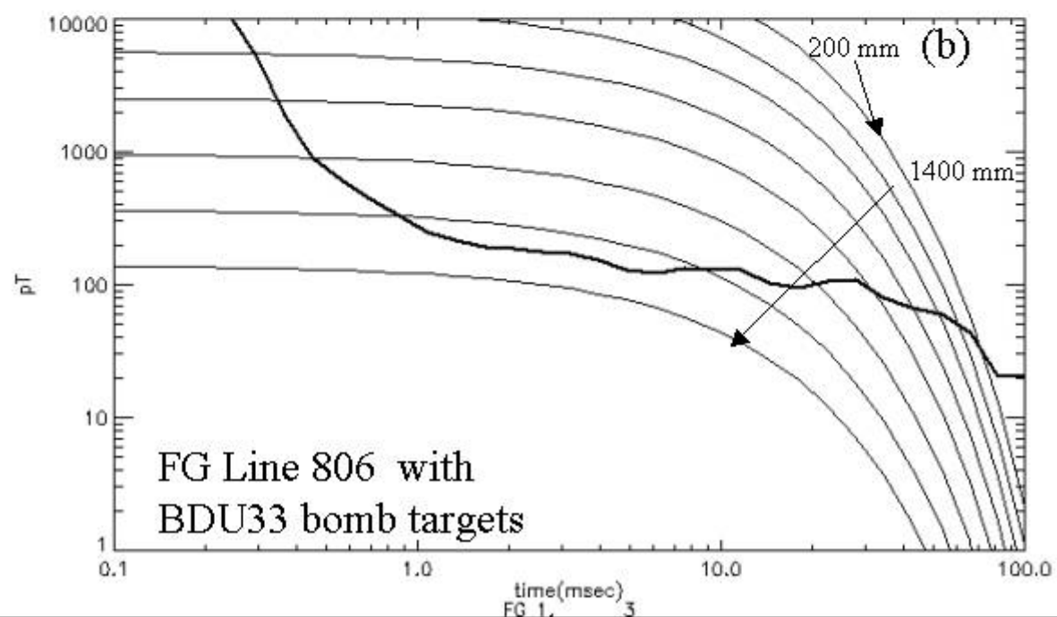
Figure 47 – Modeled response of the BDU33 practice bomb target oriented horizontally, to two EMI systems.
