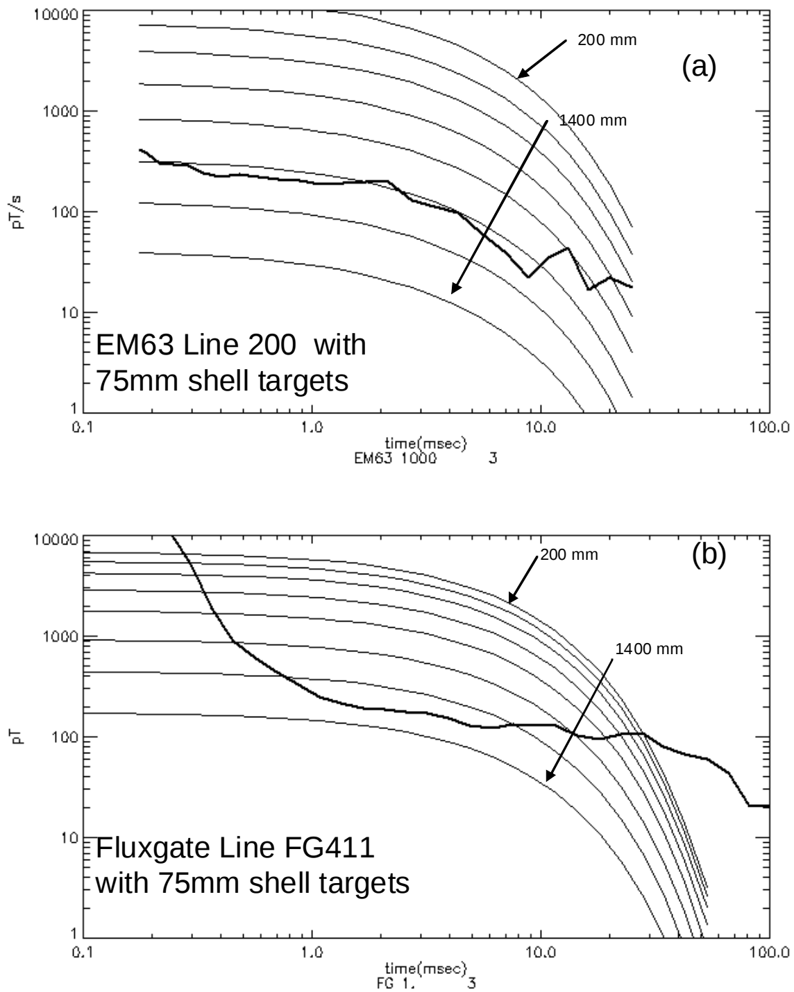
Figure 46 – Modeled response of the 75 mm shell target oriented horizontally, to two EMI systems Thick lines are observed noise levels on the EMIT test pit.
