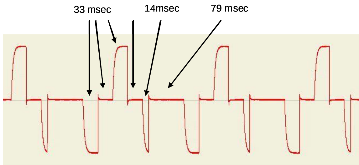
Figure 30 EM63 waveform – At 50 Hz power line setting and M frequency, measured base frequency was 4.5 Hz
