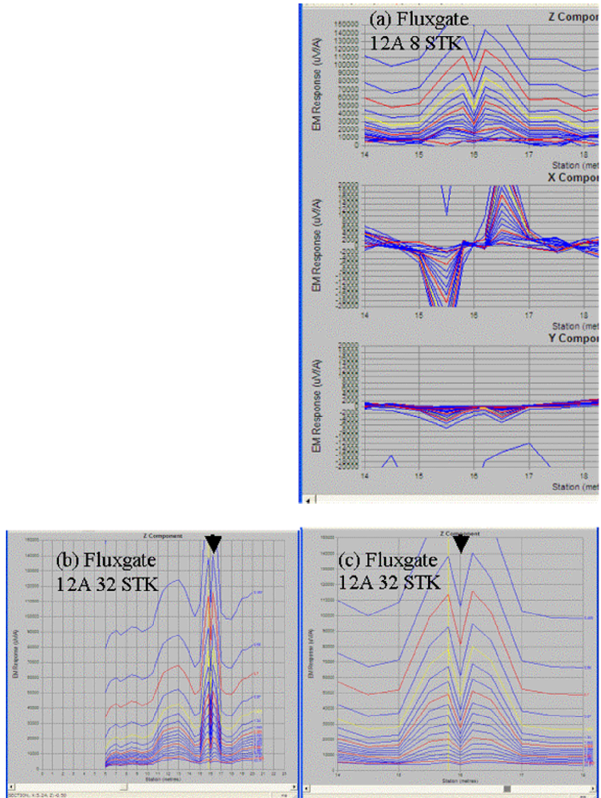
Figure 65 Three component profile acquired with the BEAMOD™ Mk2 with fluxgate sensor under power lines.
