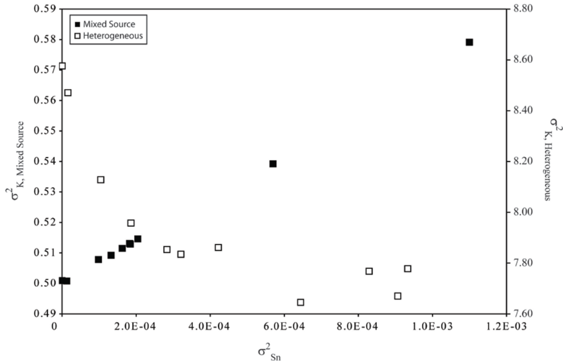
Figure 5.1.1-7. Hydraulic conductivity variance ( \sigma_K^2 ) for the Mixed-Source and Heterogeneous experiments as a function of the variance in organic-liquid saturation distribution ( \sigma_{S_n}^2 ). The variance in hydraulic conductivity and organic-liquid saturation were calculated for the entire flow cell, including organic-liquid free regions.
