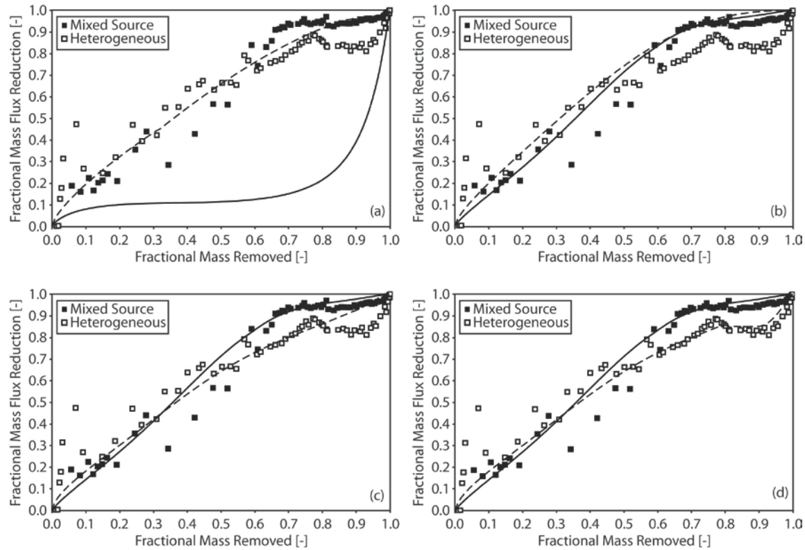
Figure 5.4-4. Mass flux reduction versus mass removal behavior for the Mixed Source and Heterogeneous experiments, and application of the various methods for characterizing mass-flux-reduction/mass-removal behavior. (a) Variable GTP method (VGTP), (b) Variable Size method (VS), (c) Multi-Domain method (MD), and (d) Multi-Domain Relative Permeability method (MDRP). The model simulations for the Mixed Source and Heterogeneous experiments are represented by the solid and dashed lines, respectively.
