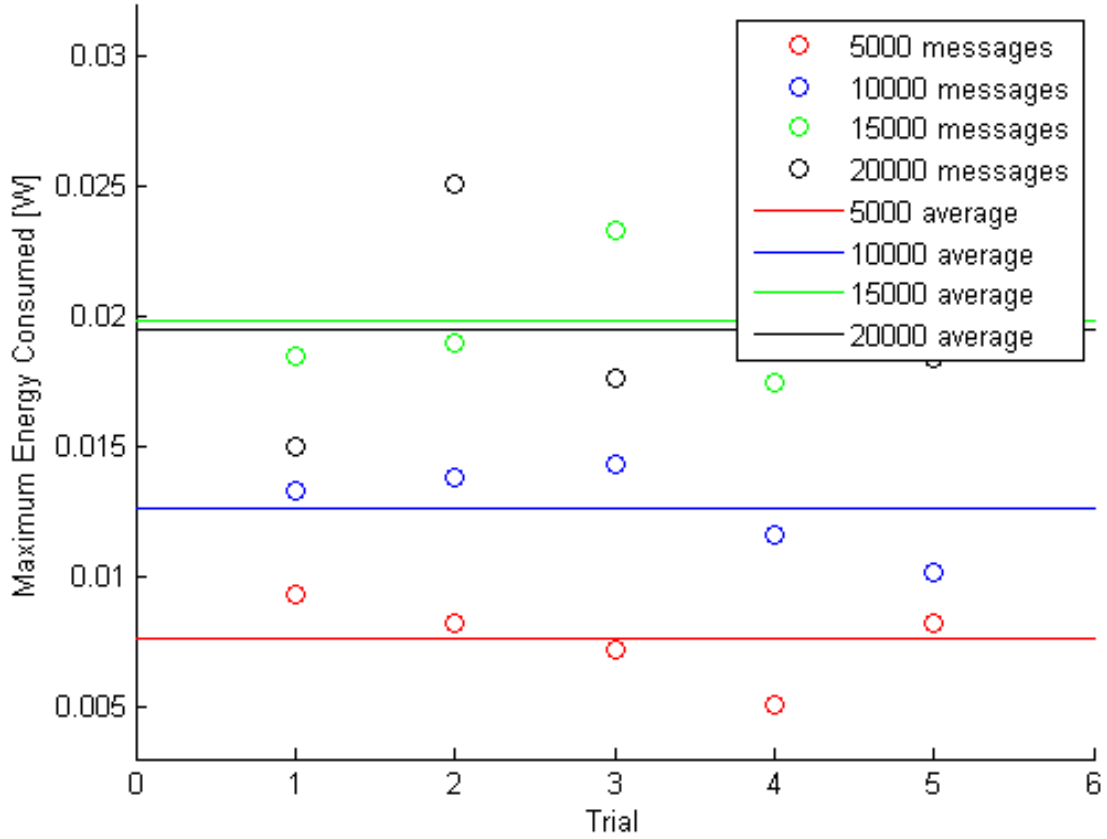
Figure 29. The maximum energy consumed by nodes in the WSN for 5,000, 10,000, 15,000, and 20,000 messages. The maximum energy consumed increases as traffic volume increases from 5,000 to 10,000 messages. The average maximum energy consumed for 15,000 messages slightly exceeds the average maximum energy consumed for 20,000 messages.
