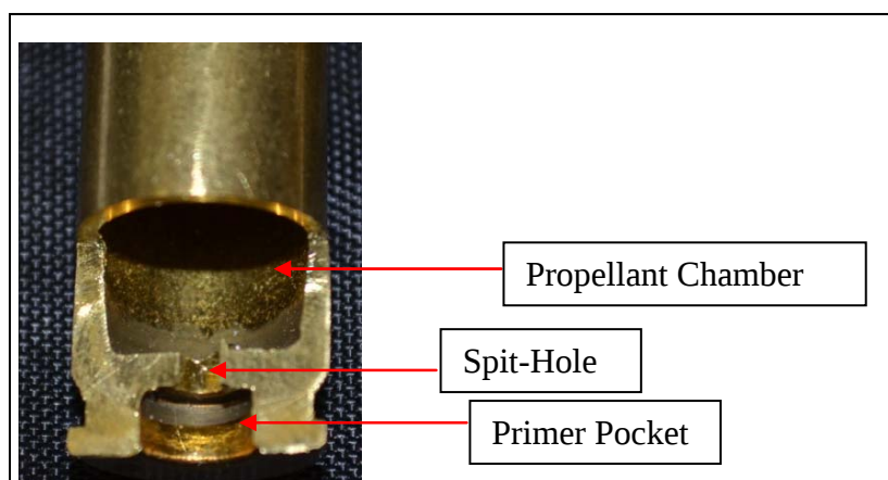
Figure 1. Standard 7.62-mm cartridge cutaway.
