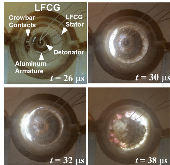
Figure 3. High-speed photographs taken during explosive and electrical operation of the LFCG.
