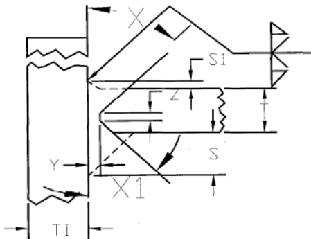
FIGURE 7. Type 7. Double-bevel-grooved tee or corner joint, double-fillet reinforced.
