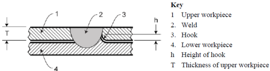
FIGURE 4 - Hook
