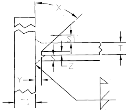
FIGURE 5. Type 5. Single-bevel-grooved corner joint, double-fillet reinforced.
