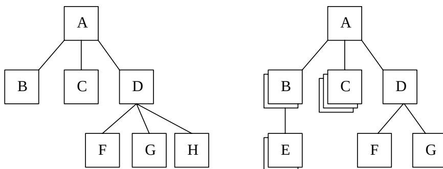
Figure 1: Jaquith user model. On the left is the current filesystem for a small disk. On the right is the corresponding Jaquith archive. The archive has multiple versions of directory B and file C , and no copy of file H . File E has been deleted from disk, but old versions are still present in the archive.
